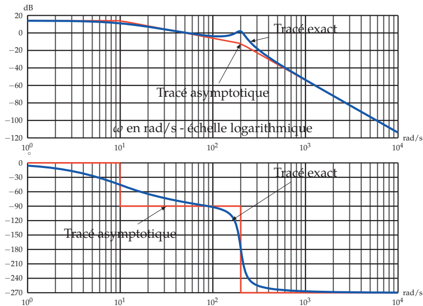
FIGURE 6.3. – Diagrammes de Bode
