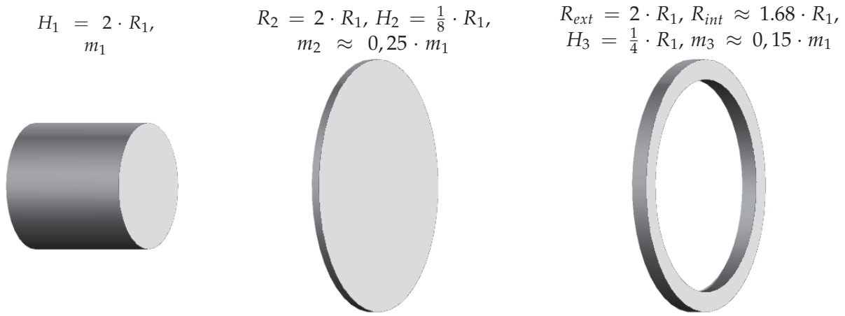
FIGURE 2.4. – Rayon de giration
